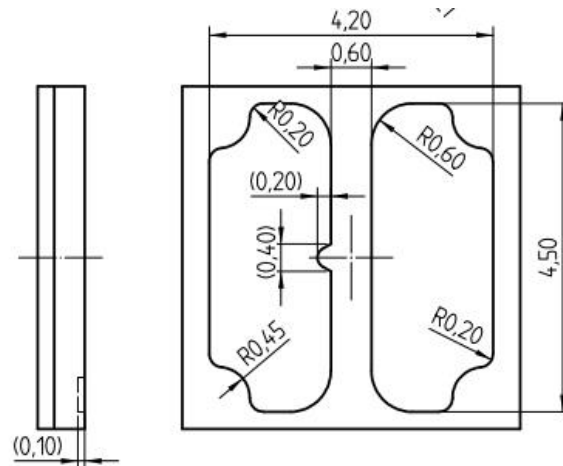
建议焊盘尺寸图 Recommended Soldering Pattern
